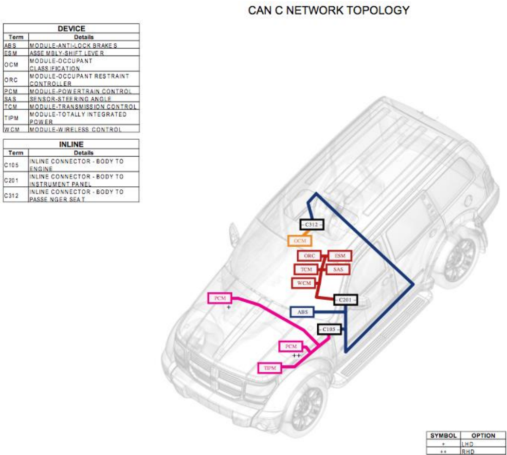
CAN-C Network – 2010 Jeep Cherokee
